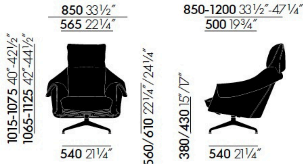
Bascule Highback, four-star base
