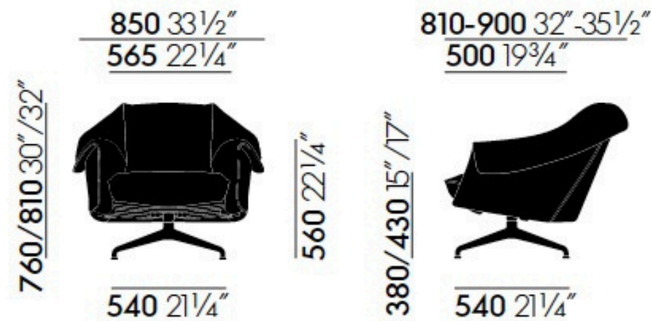
Bascule Lowback, four-star base
